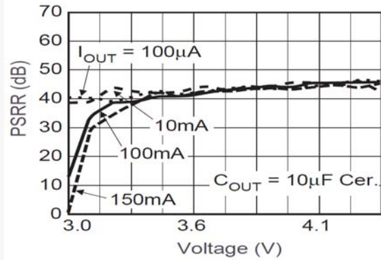
Figure 12. PSRR vs. Voltage Drop
